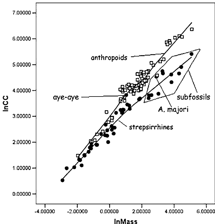
Fig. 2 Bivariate plot of logged cranial capacity (lnCC in ml) and logged body mass (lnMass in kg) in strepsirrhine primates (closed circles) and living anthropoids (open squares). The extinct giant lemurs are enclosed by a convex polygon, and nonparametric (LOESS) lines are fit to each group (tension = 0.7). Strepsirrhines fall consistently below size-matched anthropoids in brain size, although there are exceptions (e.g., the living aye-aye, Daubentonia madagascariensis , falls on the anthropoid line; Archaeolemur majori is virtually indistinguishable in its brain:body ratio from male proboscis monkeys ( Nasalis larvatus ))
