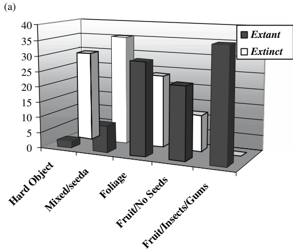
Fig. 3 Relative percentages of lemur species in each of five trophic guilds. (a) Extinct vs. extant lemurs. (b) Species living in the recent past (i.e., extinct plus extant) vs. those still extant. Data from Godfrey and Irwin (in press)
